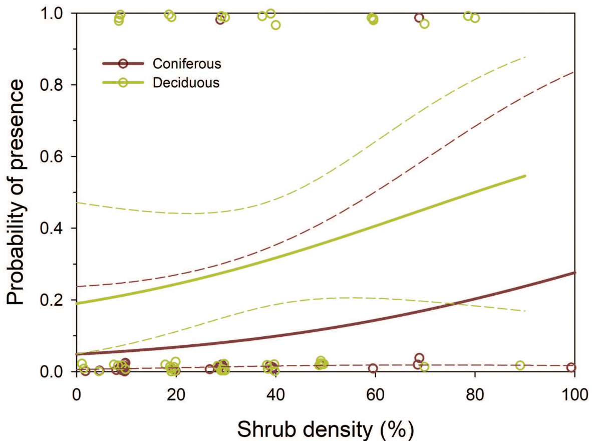
Fig. 1. Predicted probability of presence (solid lines) and 95% confidence interval (dashed lines) of Canada Warblers and percent shrub density in Lesser Slave Lake Provincial Park, Alberta. The predicted probability of Canada Warbler presence varied depending on whether a location was dominated by coniferous (red line) or deciduous (yellow line) canopy structure. The plotted range of shrub density was the minimum and maximum observed values for each canopy type while all other predictor variables were held constant at their mean observed value. The points are the observed presence-absence data.
