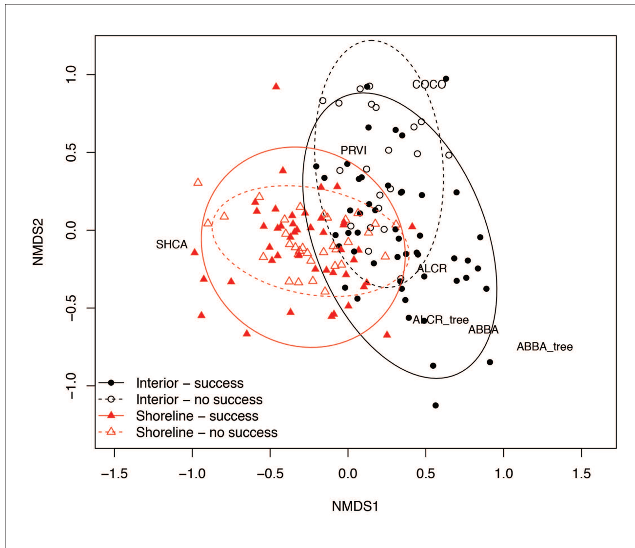
Fig. 2. Non-metric multidimensional scaling ordination of all 149 vegetation plots located within a bird territory (i.e., excluding plots surveyed outside bird territories) in woody plant species space. Symbols indicate plots in different site types ("interior" or "shoreline"), and in the territories of birds with or without evidence of nesting success ("success" or "no success"). Ellipses are the 90% confidence intervals of the multivariate distribution of each group. Select indicator species mentioned in the text are indicated: ABBA = balsam fir (shrub), ABBA_tree = balsam fir (tree), ALCR = green alder (shrub), ALCR_tree = green alder (tree), COCO = beaked hazelnut, PRVI = chokecherry, SHCA = Canada buffaloberry. Stress in three dimensions is 16.38.
